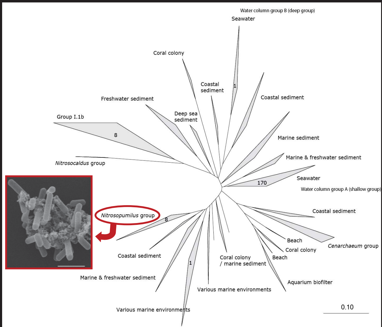
Above: Diversity of ammonia oxidizing archaea inferred by sequencing a gene ( amoA ) required for the oxidation of ammonia
